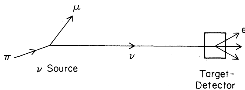
FIG. 1. A typical neutrino-oscillation experiment.
