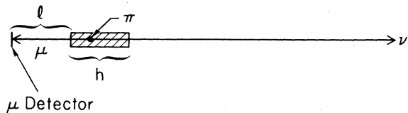
FIG. 2. A Gedankenexperiment in which pion confinement and muon detection determine the position of a neutrino, but with a residual uncertainty.
